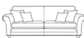
Grand sofa H 980mm W 2300mm D 1060mm
